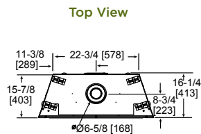
Top View Corner Installation
